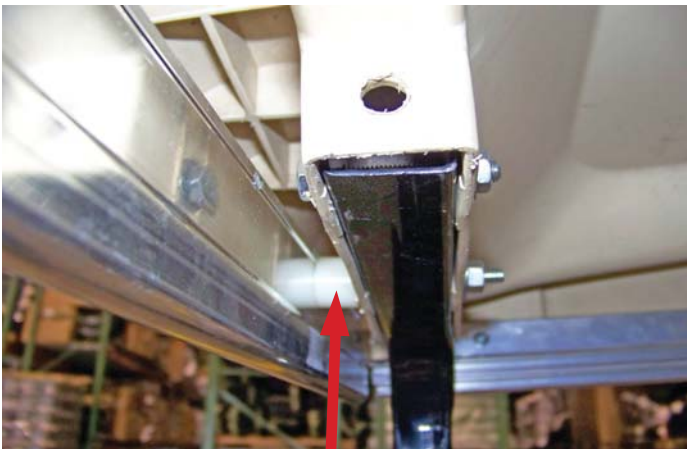
1/2" Spacer Placement
