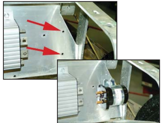
13. Solenoid Mounting
