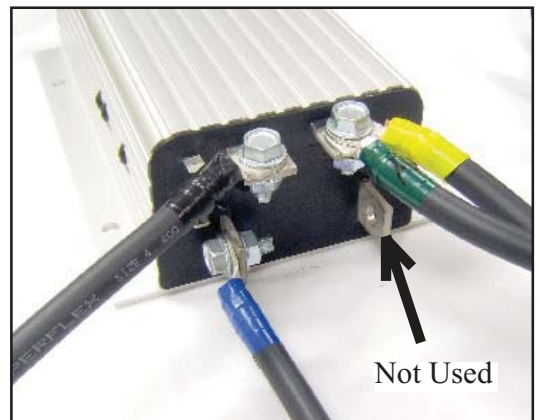
18. Black Cable Installation
