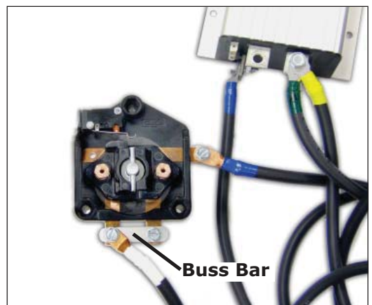
15. Blue Cable Installation
