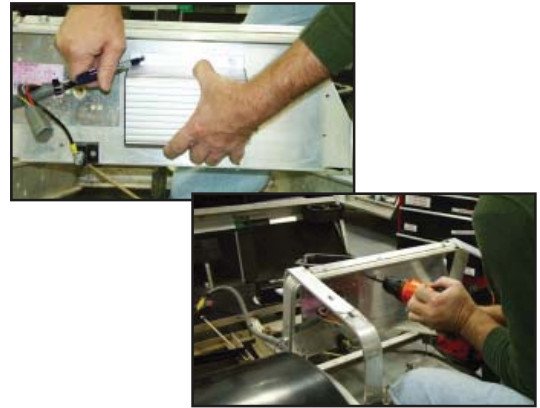
12. Controller Installation
