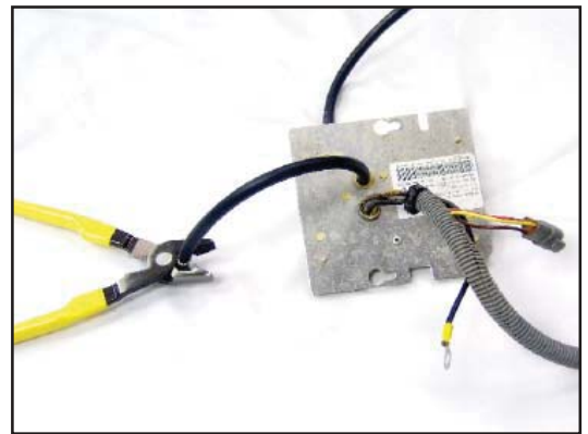
17. Black Cable Installation Through Center Hole in Computer
